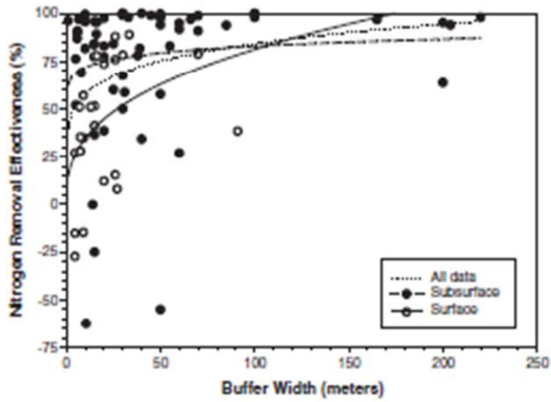
Figure 3-4. Relationship of nitrogen removal effectiveness to riparian buffer width over all studies and analyzed by water flow path. Lines are fitted to model y = ax^b . (Mayer et al., 2007)
