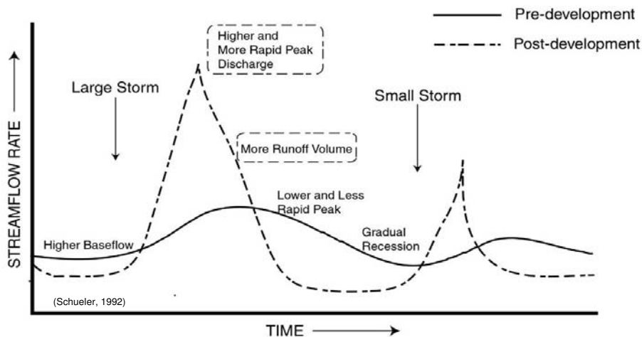
Figure 1. Changes in hydrology after development (Schueler 1987).
