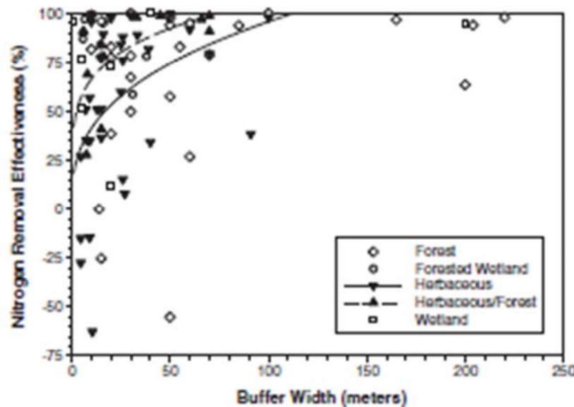
Figure 3-5. Relationship of nitrogen removal effectiveness to riparian buffer width analyzed by vegetation type. Lines are fitted to model y = ax^b . Only the regression lines for herbaceous and herbaceous/forest vegetation types are shown because model results for other vegetation types were not significant ( P > .3 ). (Mayer et al., 2007)
