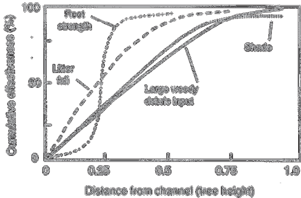
Figure 3-2. The cumulative effectiveness of various functions of riparian vegetation in relation to distance from the streambank in western Oregon. [Murphy (1995) after FEMAT 1993]. For San Juan County, the height of mature conifers is estimated to be 80 – 90 feet.
