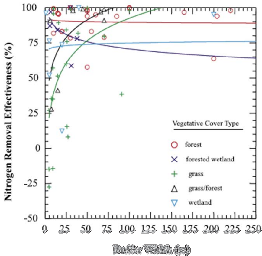
Figure 3-8. Relationship of nitrogen removal effectiveness to riparian buffer width by riparian vegetation type. Curves are fitted to non-linear model: y = a * \ln(x) + b . (Mayer et. al , 2005).
