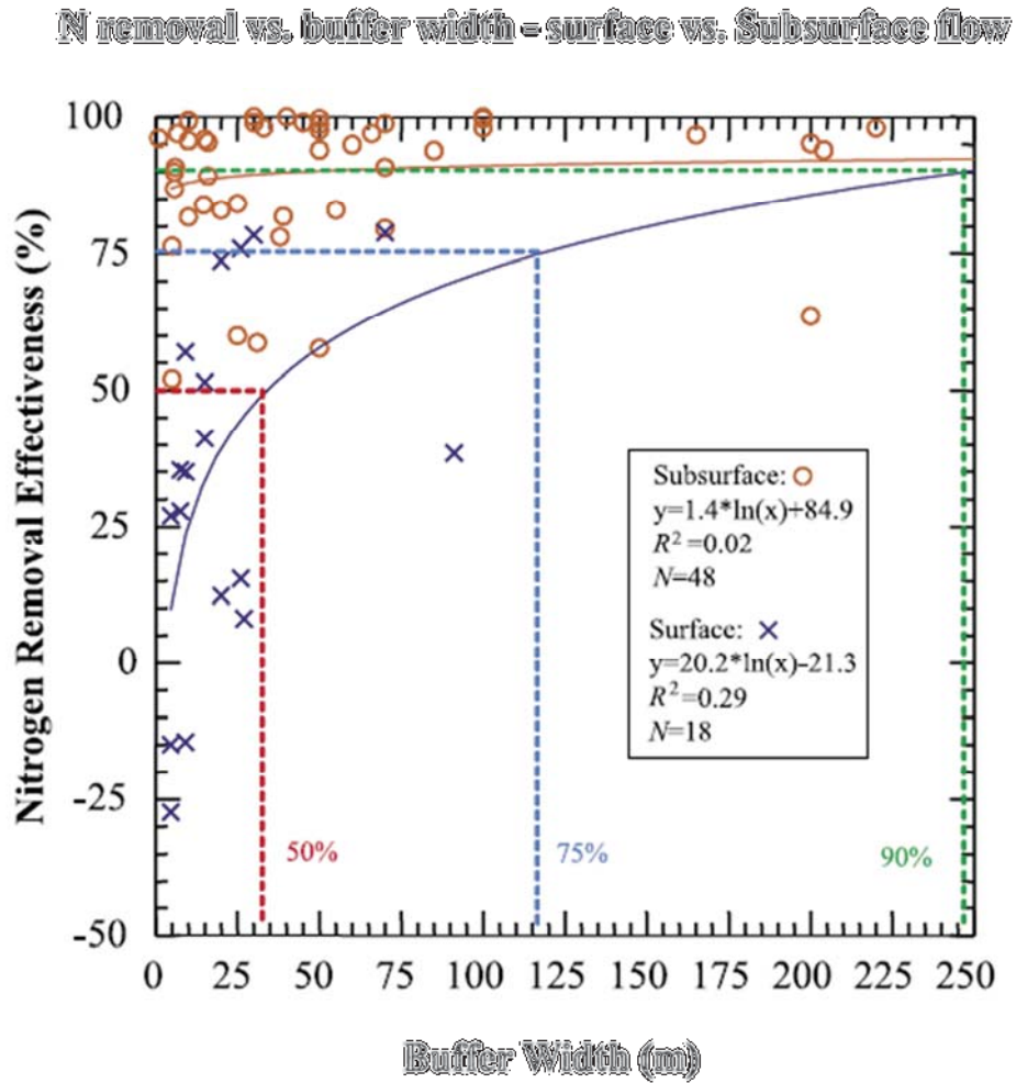
Figure 3-7. Relationship of nitrogen removal effectiveness to riparian buffer width by flow path. Lines indicate probable 50%, 75% and 90% nitrogen removal efficiencies in the surface flow path based on the fitted non-linear model (Mayer et al., 2005).
